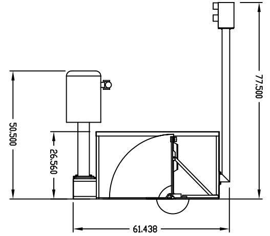
890 SURFACE MOUNT BARRIER 10' LEFT HAND ASSEMBLY
